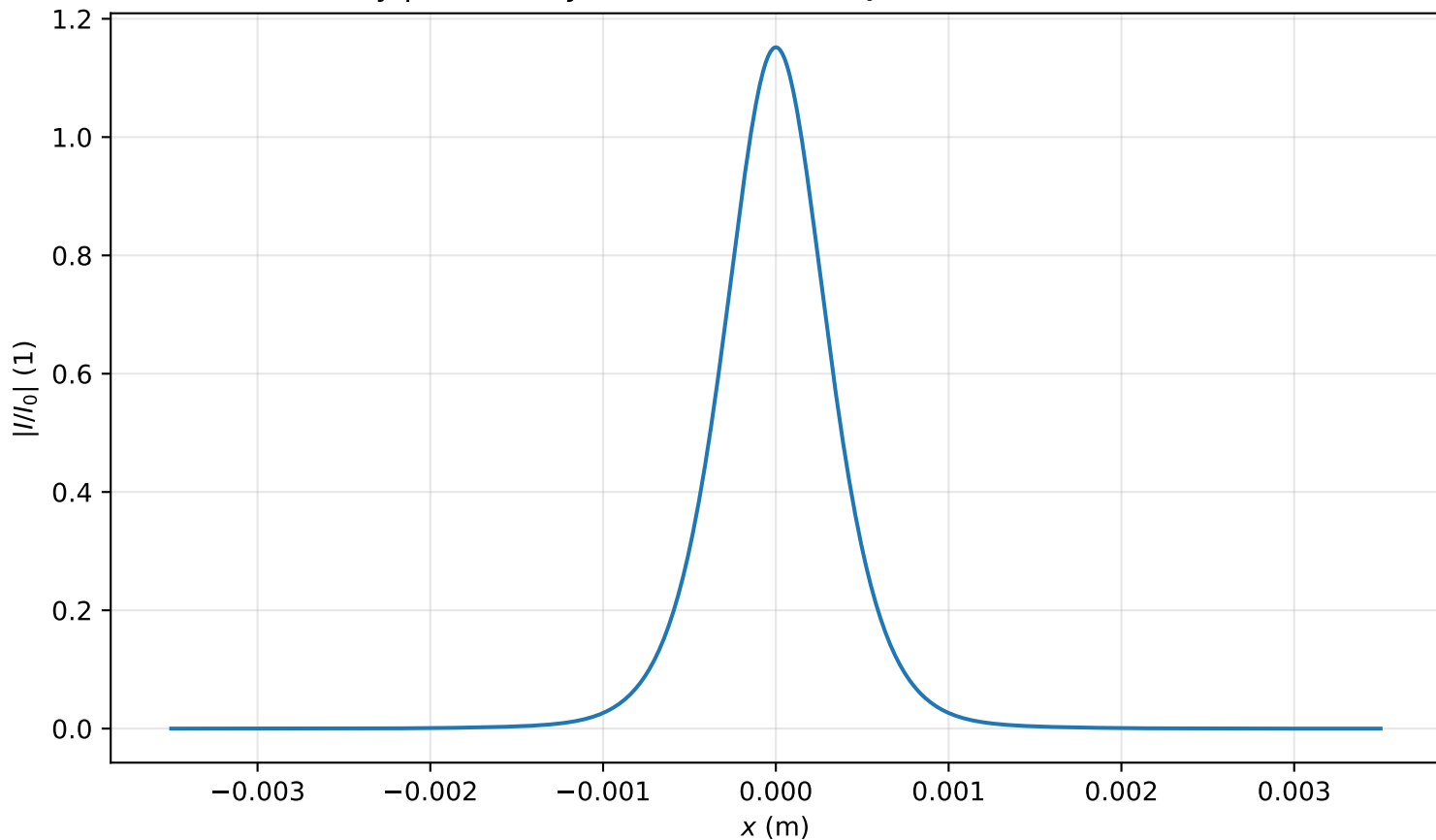
Intensity profile I(x, y = 0, z = 2.786m)/I_0 , P_{in}=0.8P_{cr} , artificial time
